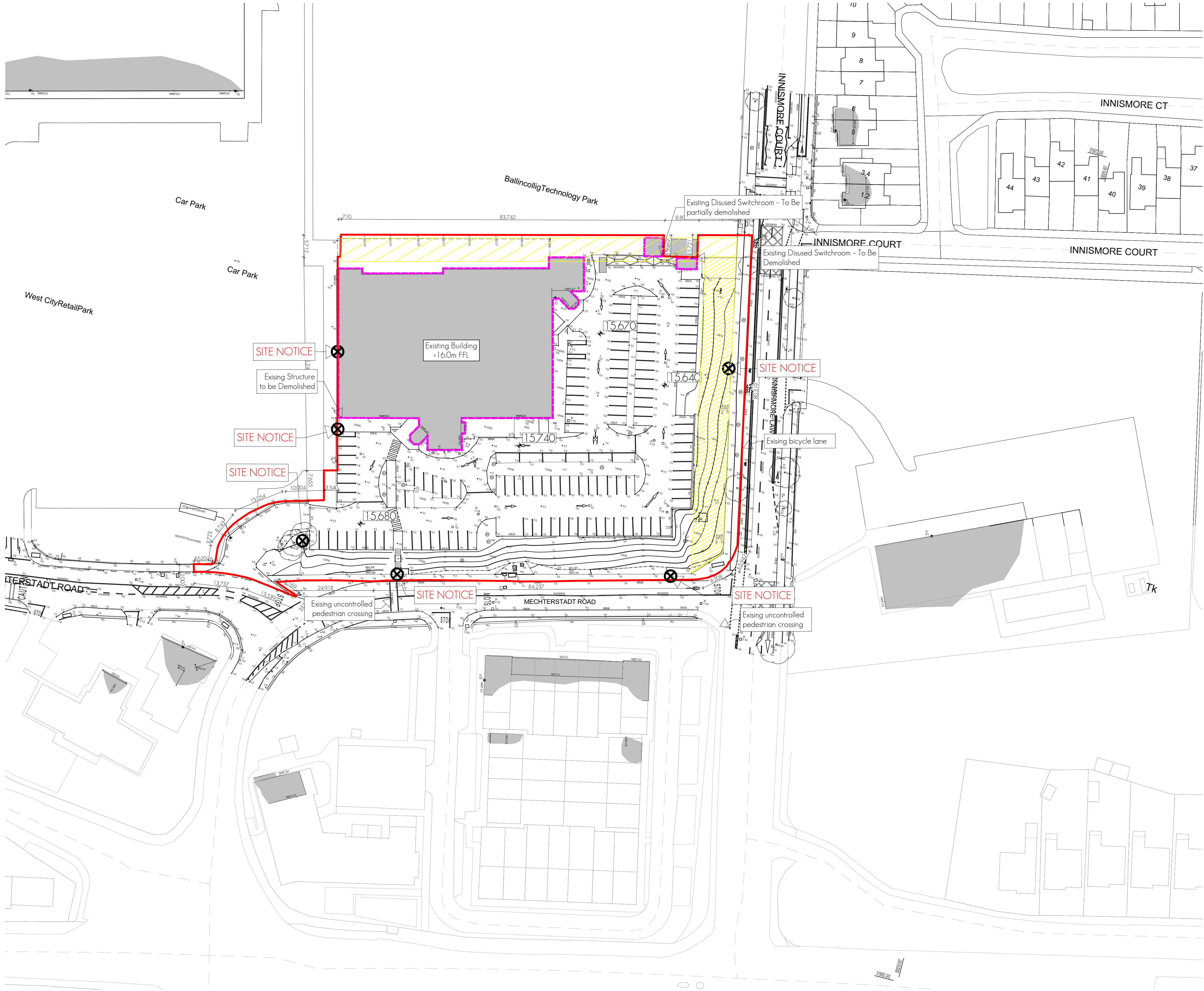
Existing Site Layout (1:500) 1:500
